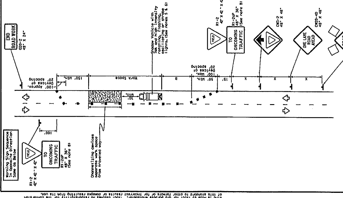
TCP (1-20) ONE LANE TWO-WAY CONTROL WITH YIELD SIGNS (Less than 2000 ADT - See note 7)
